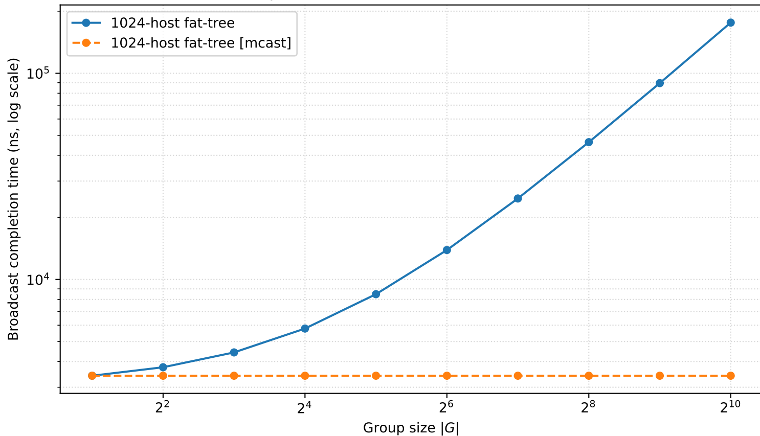
Broadcast completion: baseline vs multicast (1024-host fat tree)
