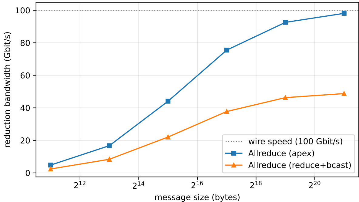
Aggregation bandwidth vs message size ( |G|=8 )
