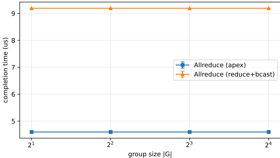
Aggregation completion vs |G| (16-host fat tree, 16 KiB)
