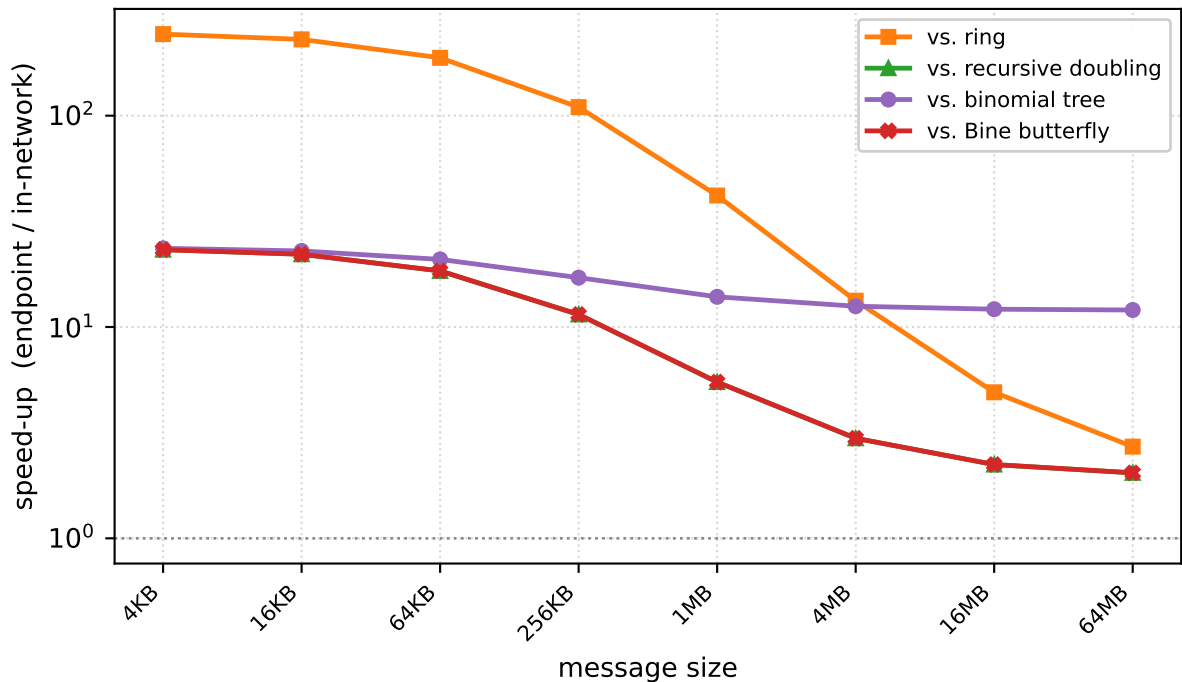
AllReduce, |G| = 64 , single-switch (pcm-sdk, measured)
