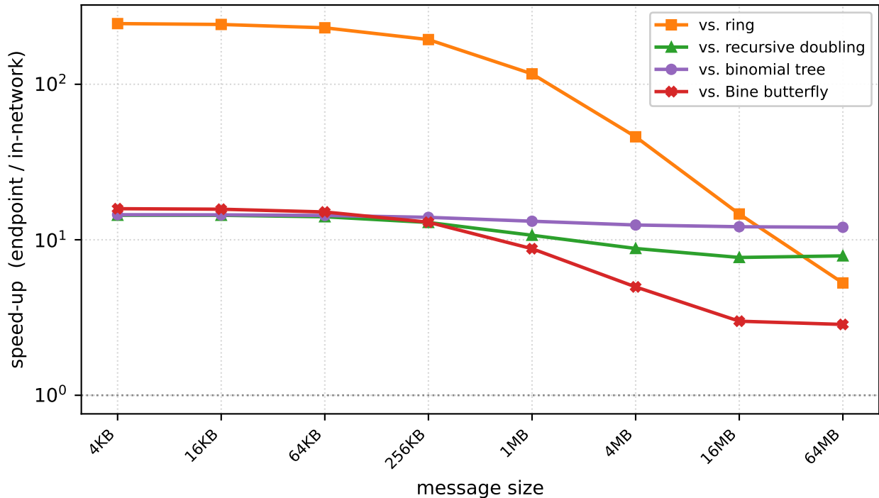
AllReduce, |G| = 64 , scaleup_3tier_64_oversub4_4000Gbps (pcm-sdk, measured)
