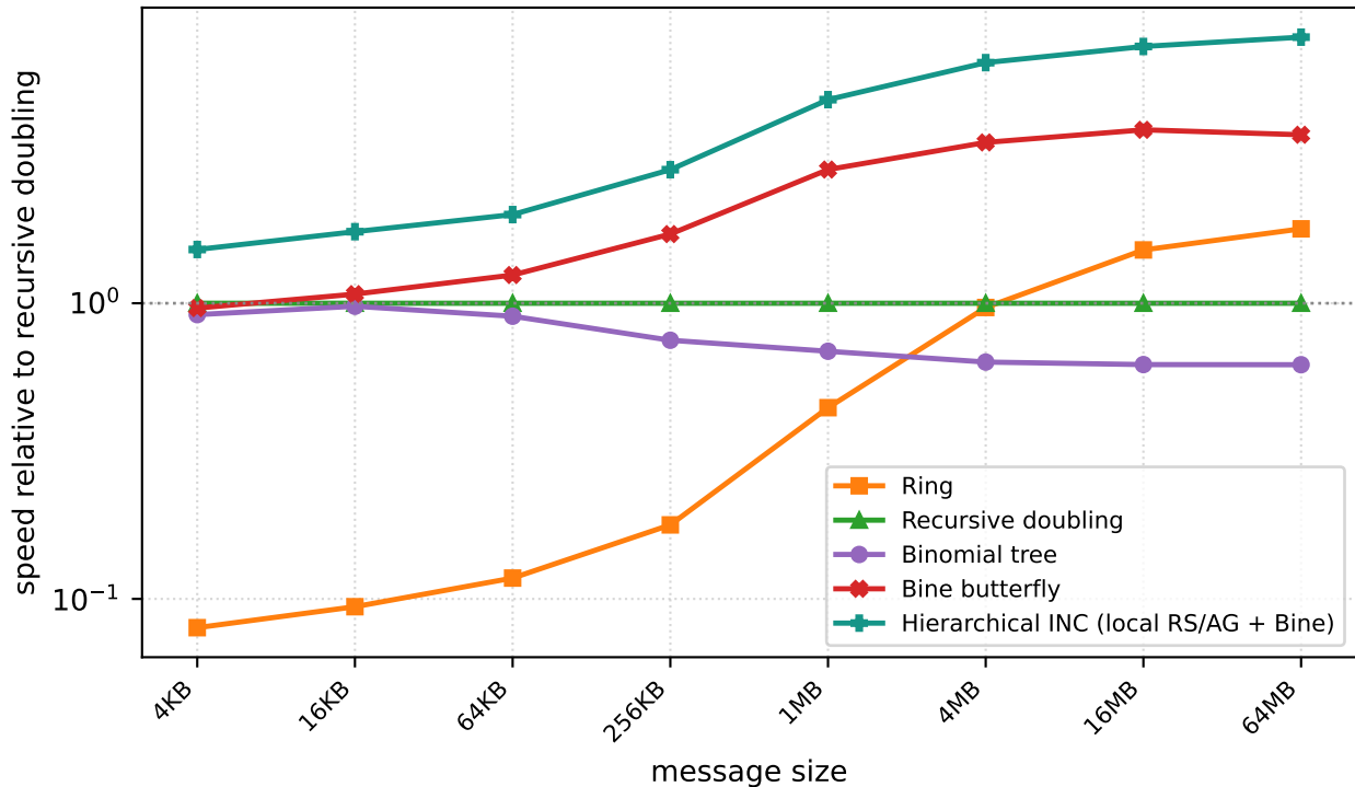
Scale-out AllReduce, |G|=64 (8 x 8-GPU domains)
