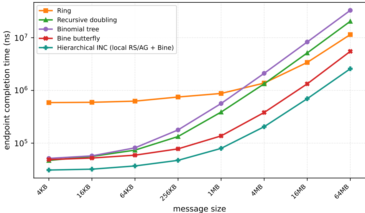
AllReduce, |G|=64 (8 x 8-GPU domains), scaleout_2tier_64_oversub2_100Gbps
