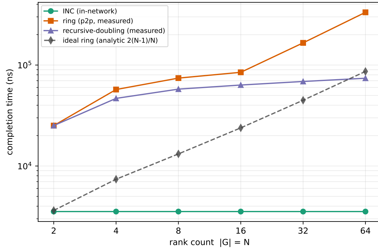
Completion vs N (1MiB/rank)
