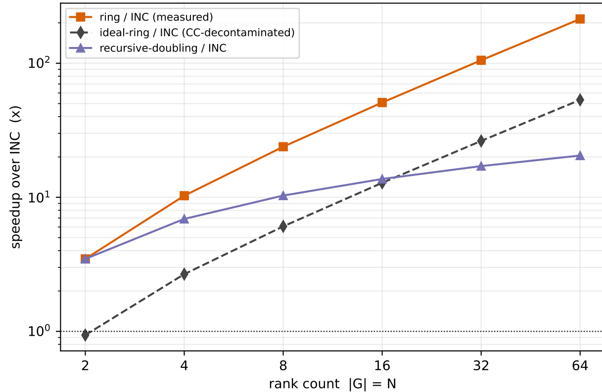
INC speedup vs N (1MiB/rank)
