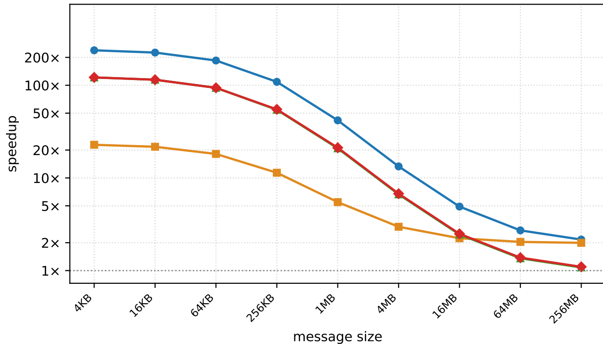
single-switch crossbar
