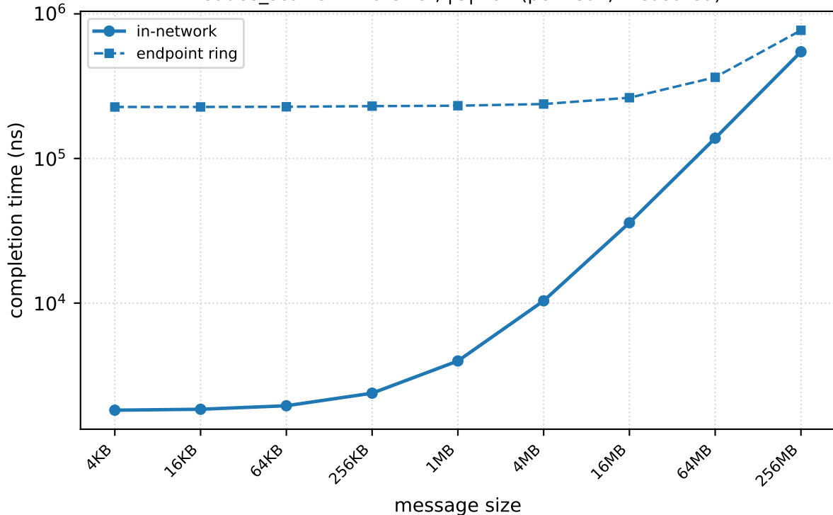
reduce_scatter — fat3tier, |G|=64 (pcm-sdk, measured)
