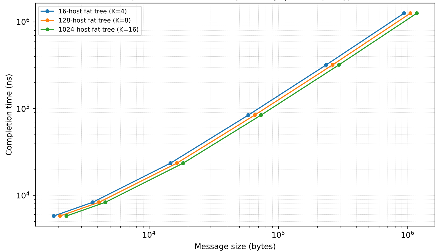
Baseline completion time vs message size ( |G|=16 , topology-invariant)
