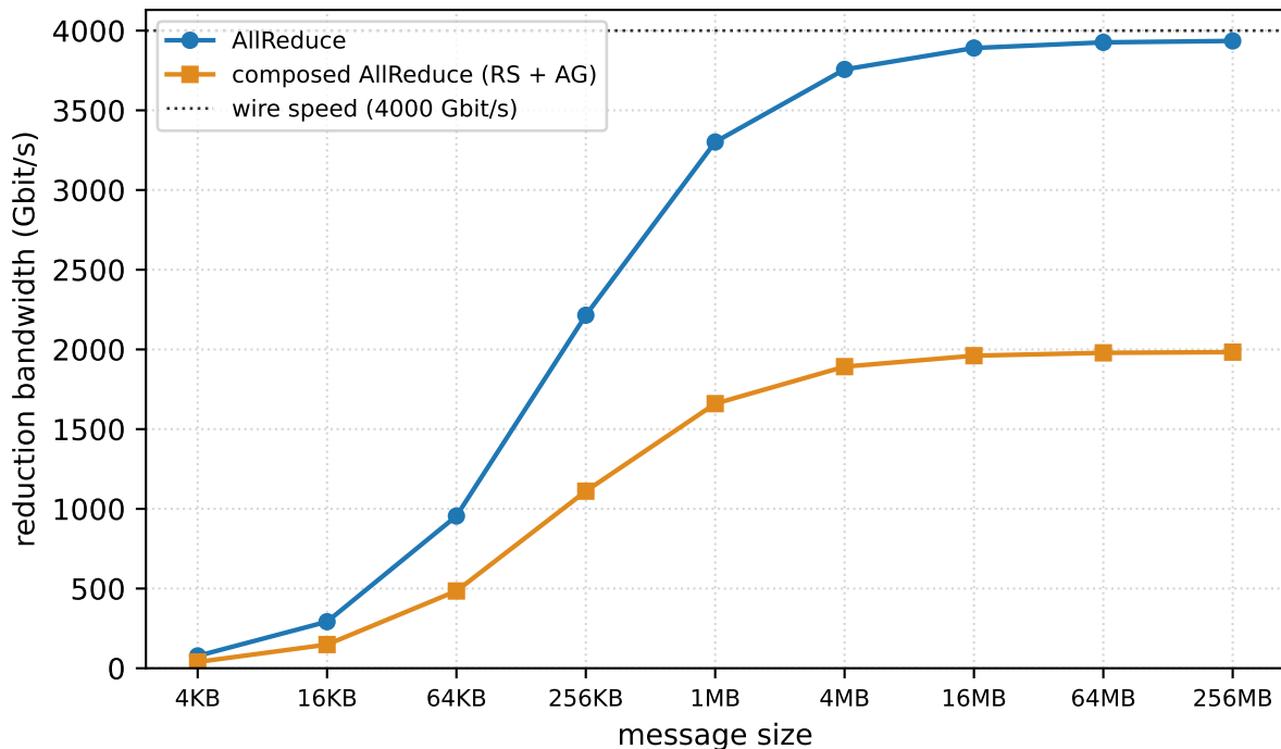
AllReduce reduction bandwidth: switch turnaround vs composed (RS + AG) ( |G|=64 , pcm-sdk, measured)
