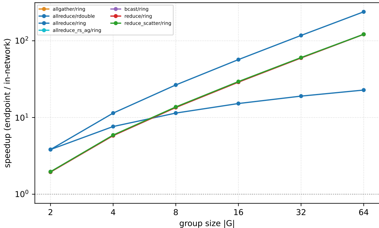
Speed-up vs |G| — 4 KiB (pcm-sdk, single-switch, measured)
