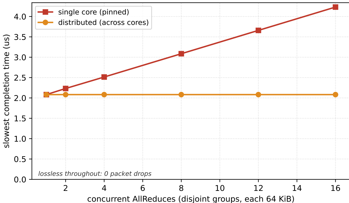
Lossless backpressure: one core serialises, many cores share (pcm-sdk, 256-host 3-tier fat-tree, measured)
