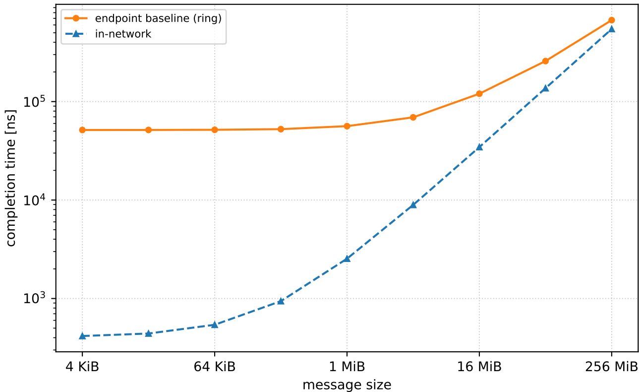
Broadcast, |G| = 64 , single-switch
