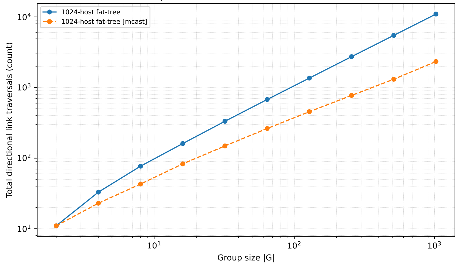
Network footprint: baseline vs multicast (1024-node fat tree)
