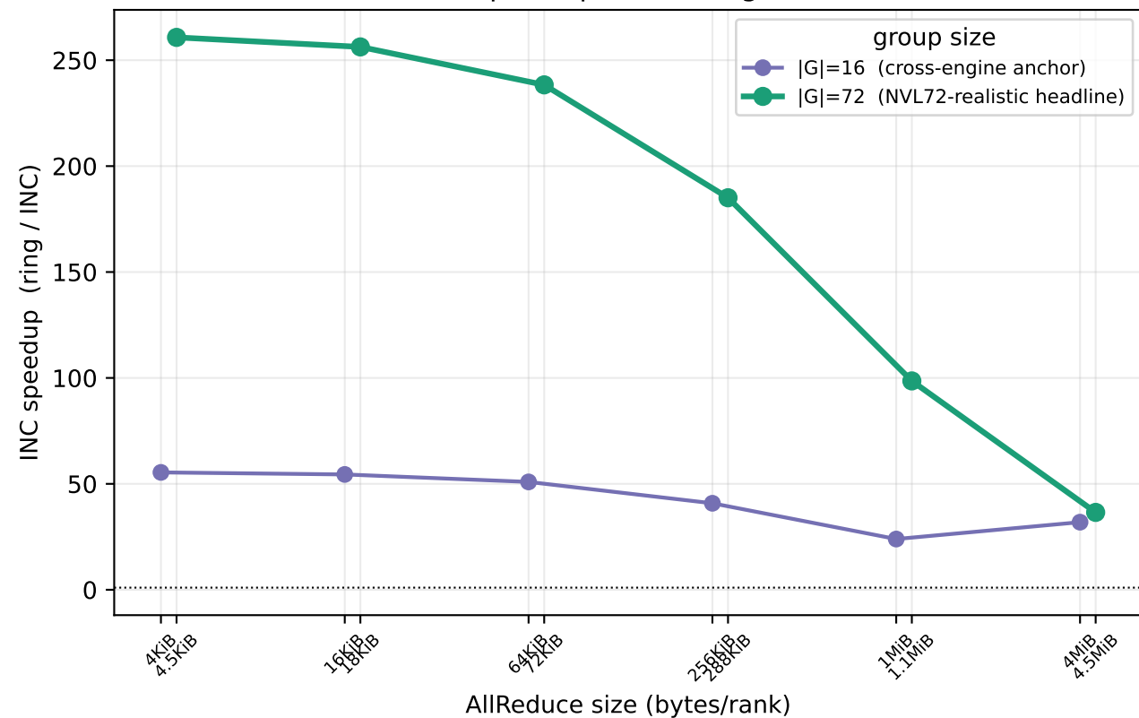
INC speedup vs message size
