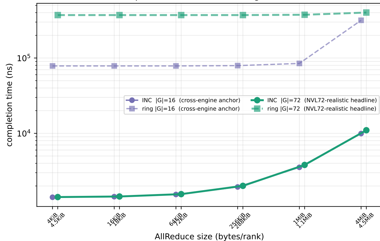
Completion: INC (solid) vs ring (dashed)
