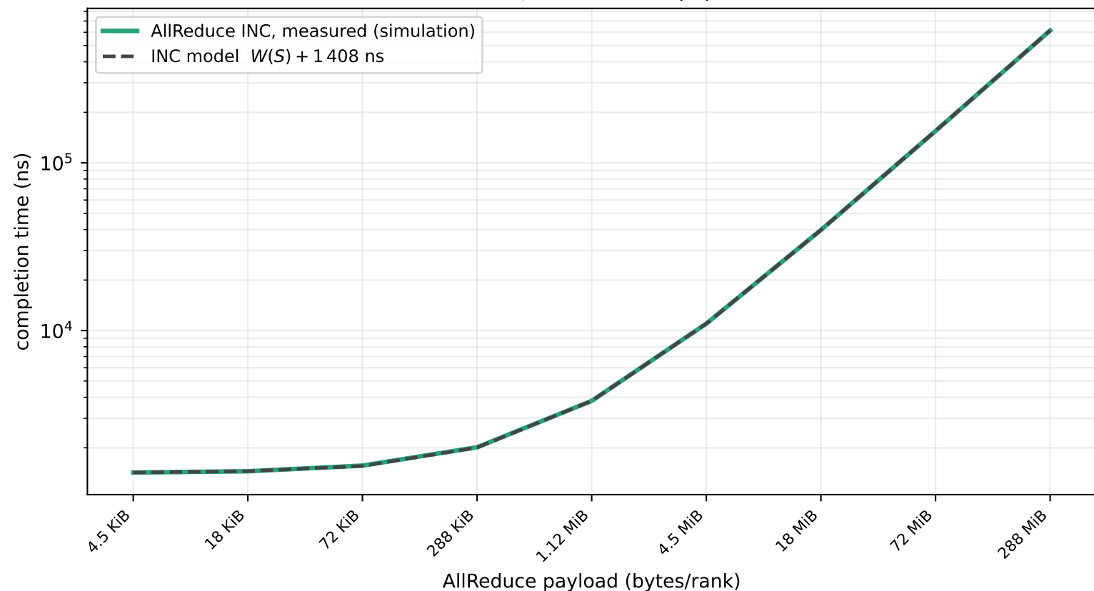
AllReduce INC, measured vs analytic model at |G| = 72 (worst residual 0.51%)
