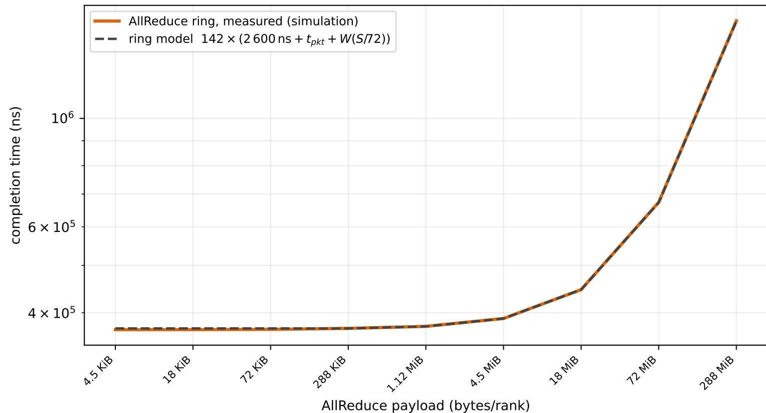
AllReduce ring, measured vs analytic model at |G| = 72 (worst residual 0.61%)
