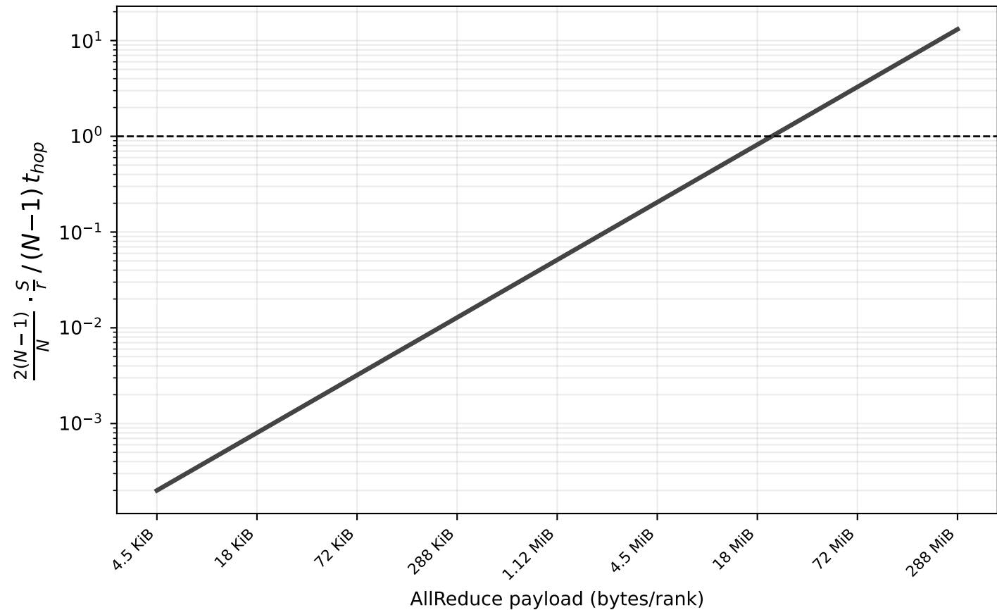
Ideal ring at |G| = 72 : bandwidth term / latency term
