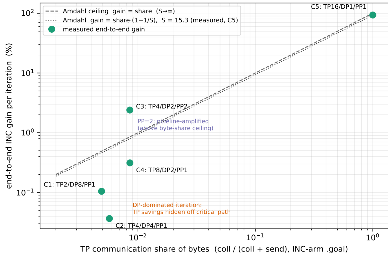
llama3 16-rank two-tier A/B: end-to-end INC gain vs TP share scale-out tree16 (100 Gbps, lossy) + per-node single-switch scale-up (3600 Gbps, lossless PFC)
