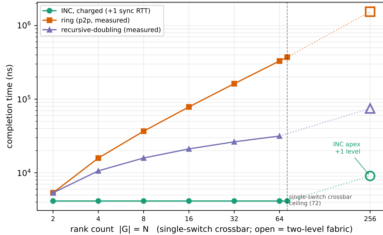
Completion vs N (1MiB/rank)
