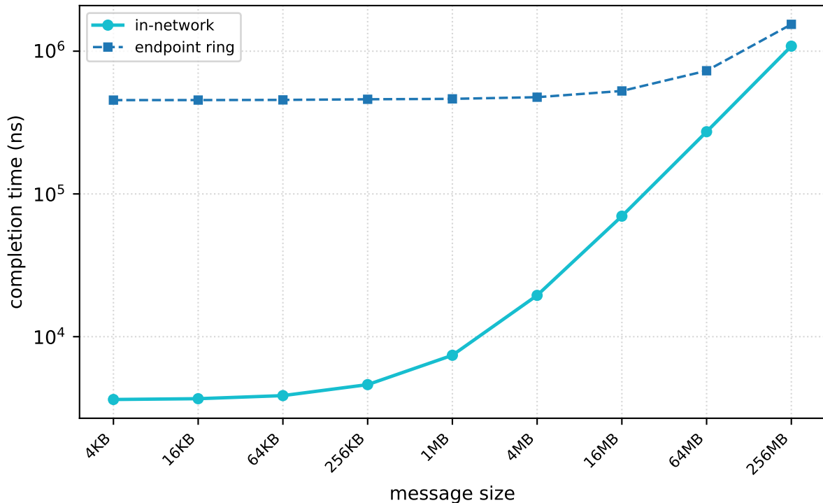
allreduce_rs_ag — fat3tier, |G|=64 (pcm-sdk, measured)
