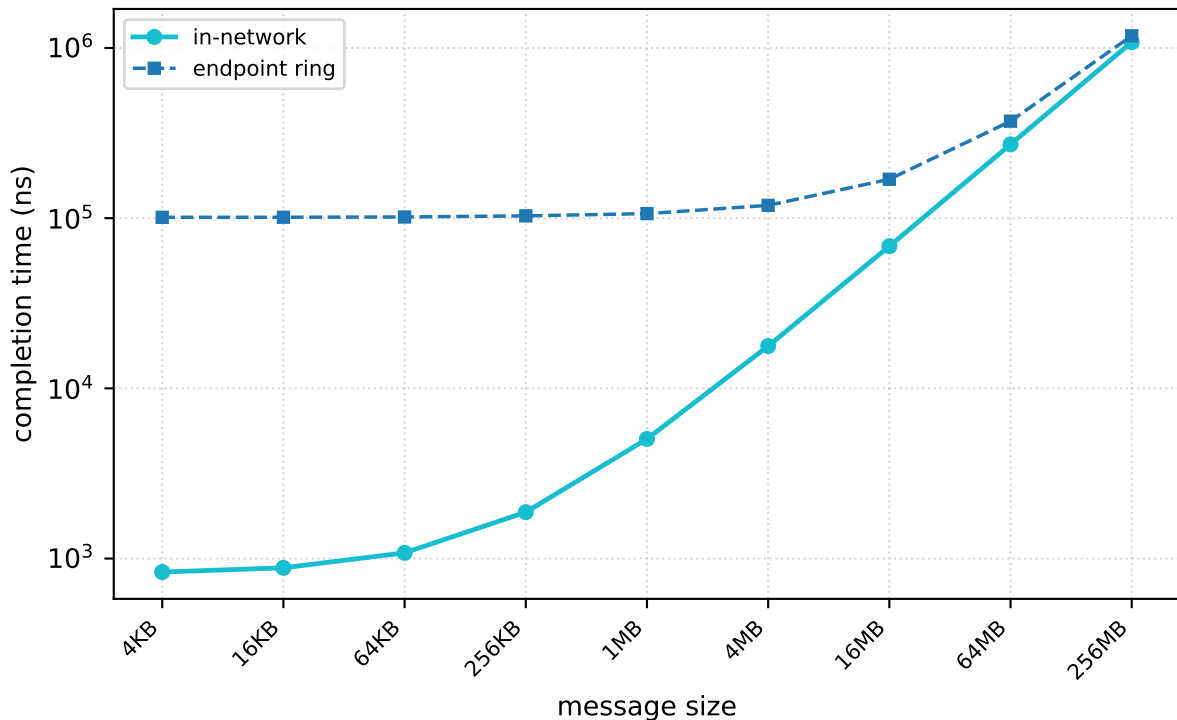
allreduce_rs_ag — single_switch, |G|=64 (pcm-sdk, measured)
