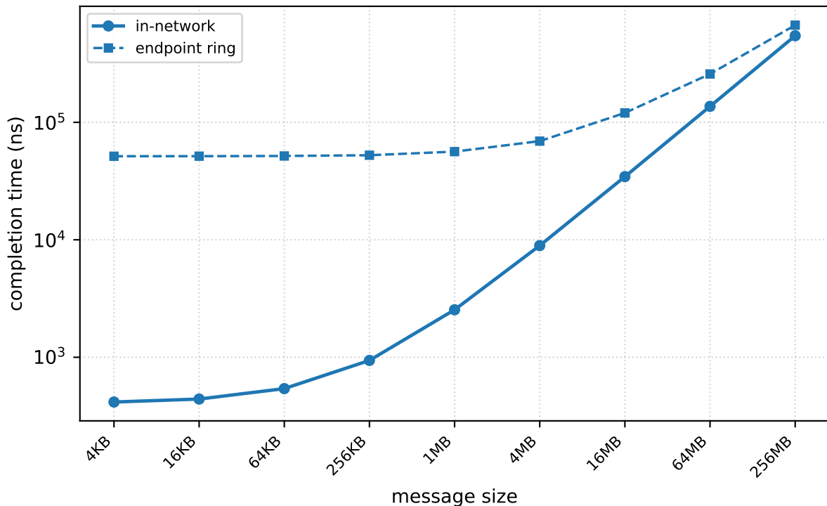
bcast — single_switch, |G|=64 (pcm-sdk, measured)
