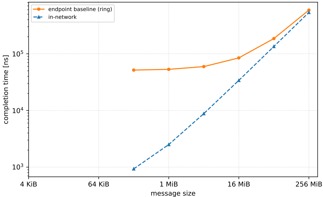
AllGather, |G| = 64 , single-switch
