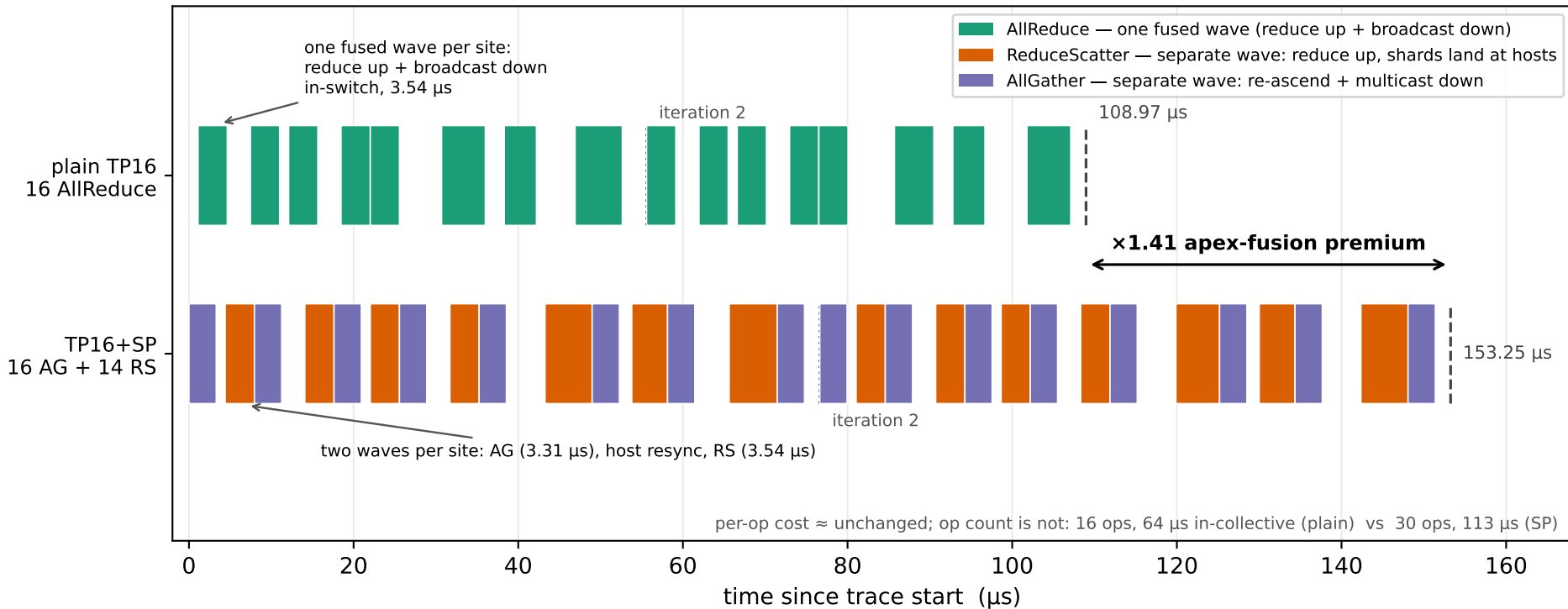
C5 INC arms op by op: monolithic AllReduce vs its SP re-rendering (ReduceScatter+AllGather) 16 ranks, 1 MiB per collective, 2 iterations — single-switch scale-up (3600 Gbps, lossless PFC), pcm-sdk two-tier
