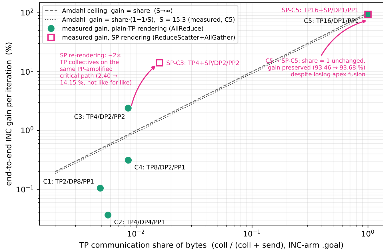
llama3 16-rank two-tier A/B: INC gain vs TP share, plain-TP vs SP rendering scale-out tree16 (100 Gbps, lossy) + per-node single-switch scale-up (3600 Gbps, lossless PFC)
