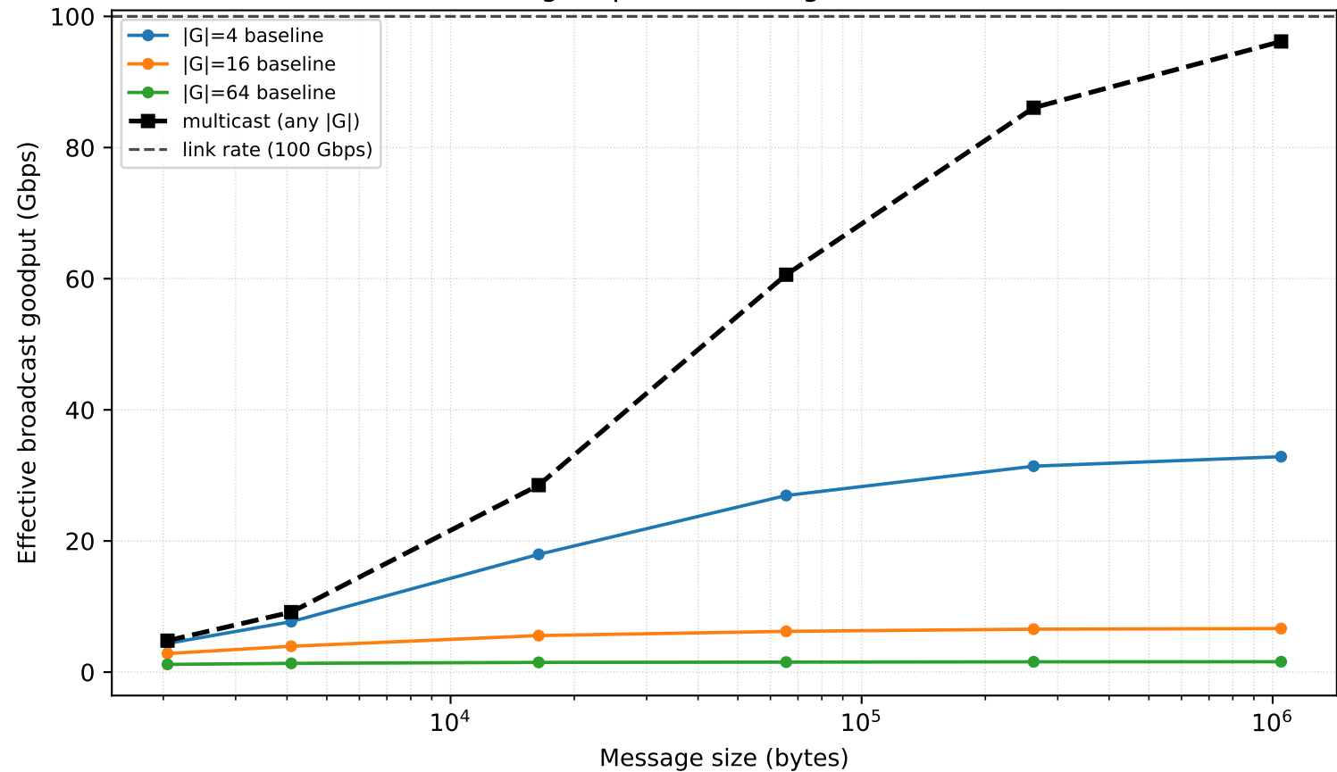
Effective broadcast goodput vs message size (1024-host fat tree)
