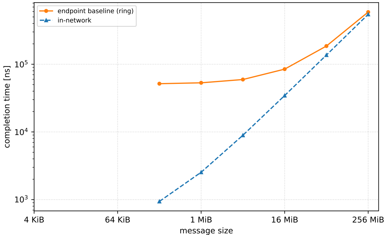
Reduce-Scatter, |G| = 64 , single-switch
