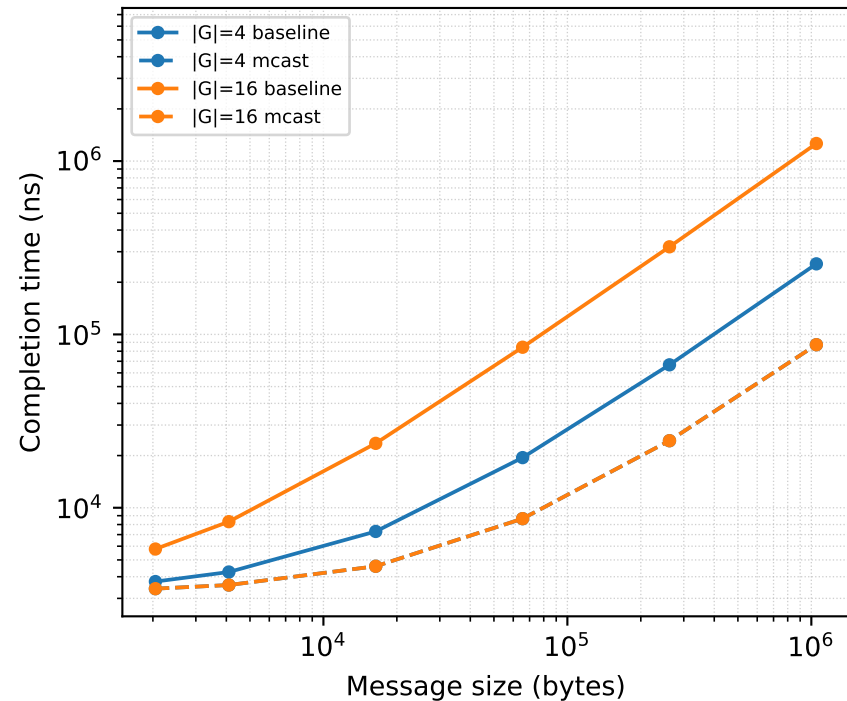
16-host fat tree (K=4)
