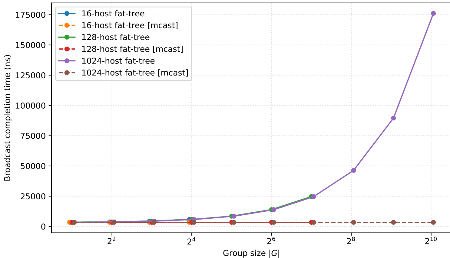
Broadcast completion time: baseline vs multicast (median)
