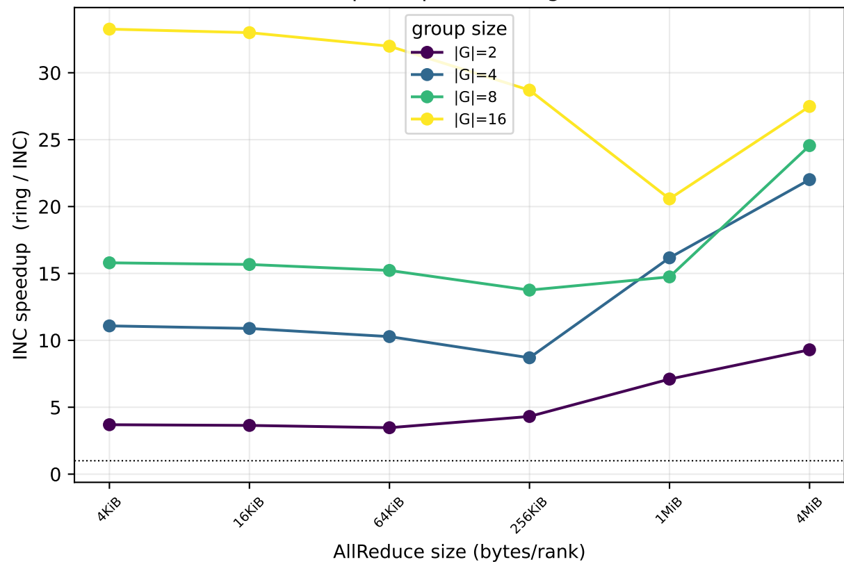
INC speedup vs message size
