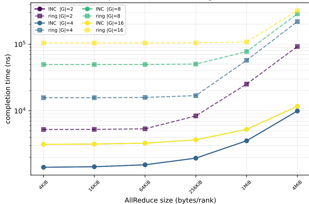
Completion: INC (solid) vs ring (dashed)
