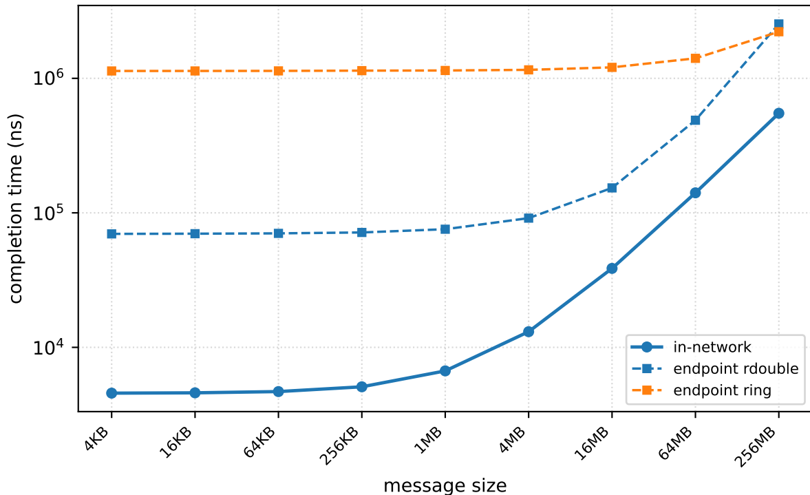
allreduce — fat3tier, |G|=64 (pcm-sdk, measured)
