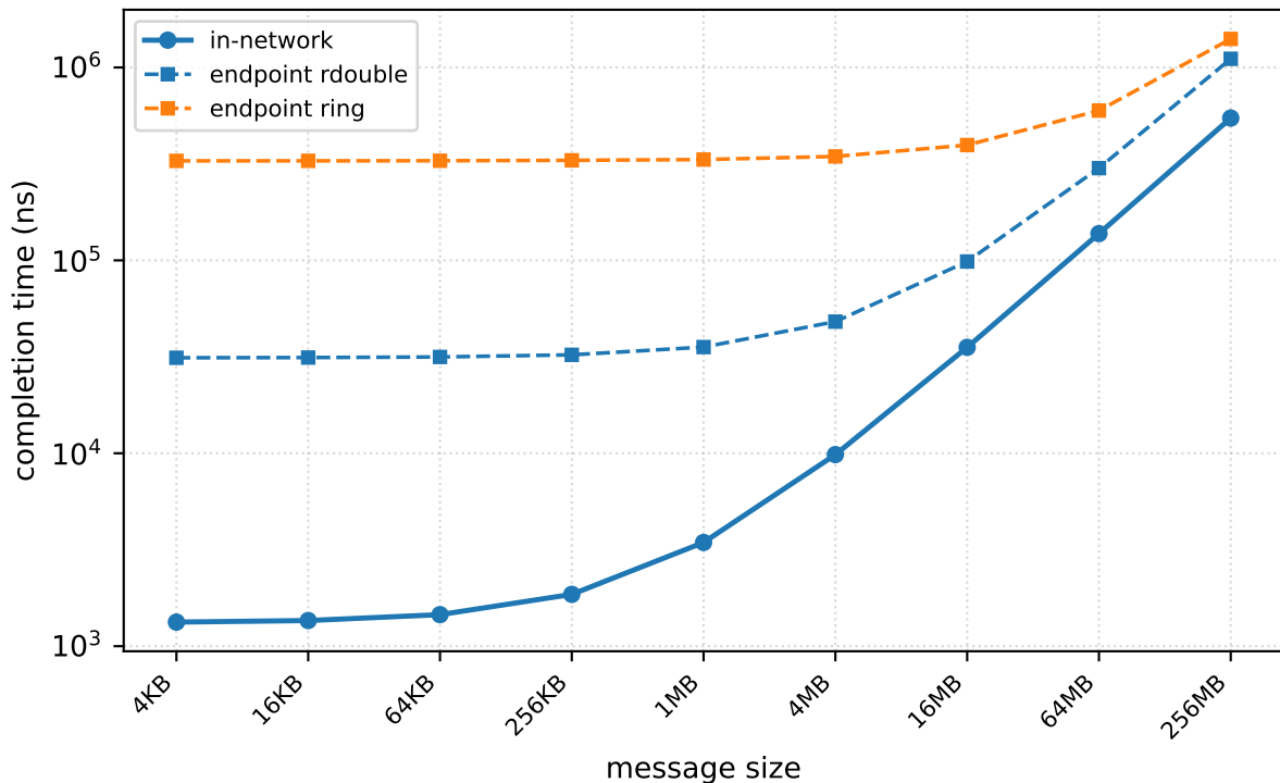
allreduce — single_switch, |G|=64 (pcm-sdk, measured)
