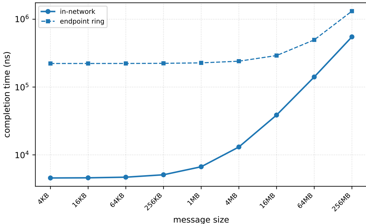
bcast — fat3tier, |G|=64 (pcm-sdk, measured)
