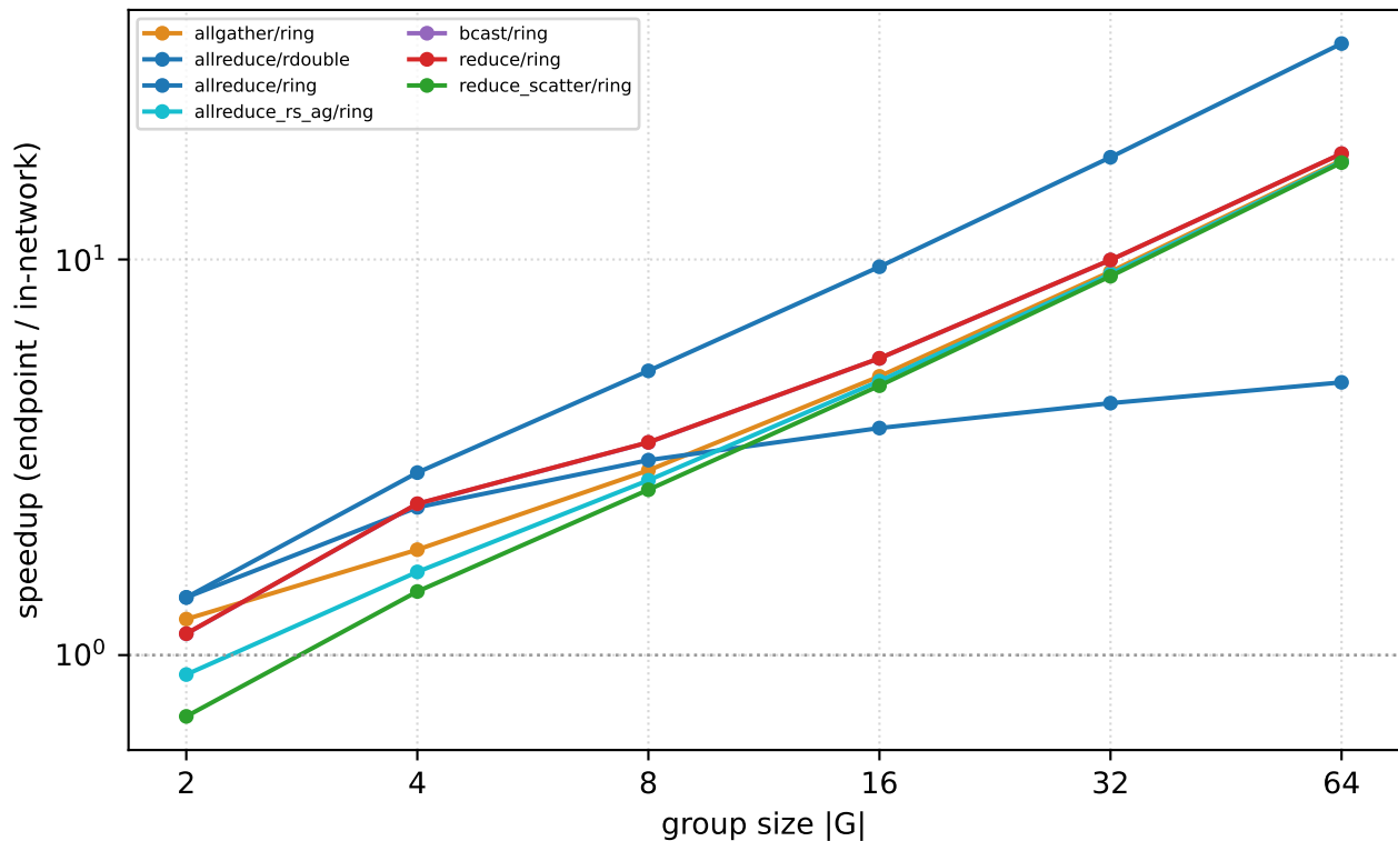
Speed-up vs |G| — 4 MiB (pcm-sdk, single-switch, measured)
