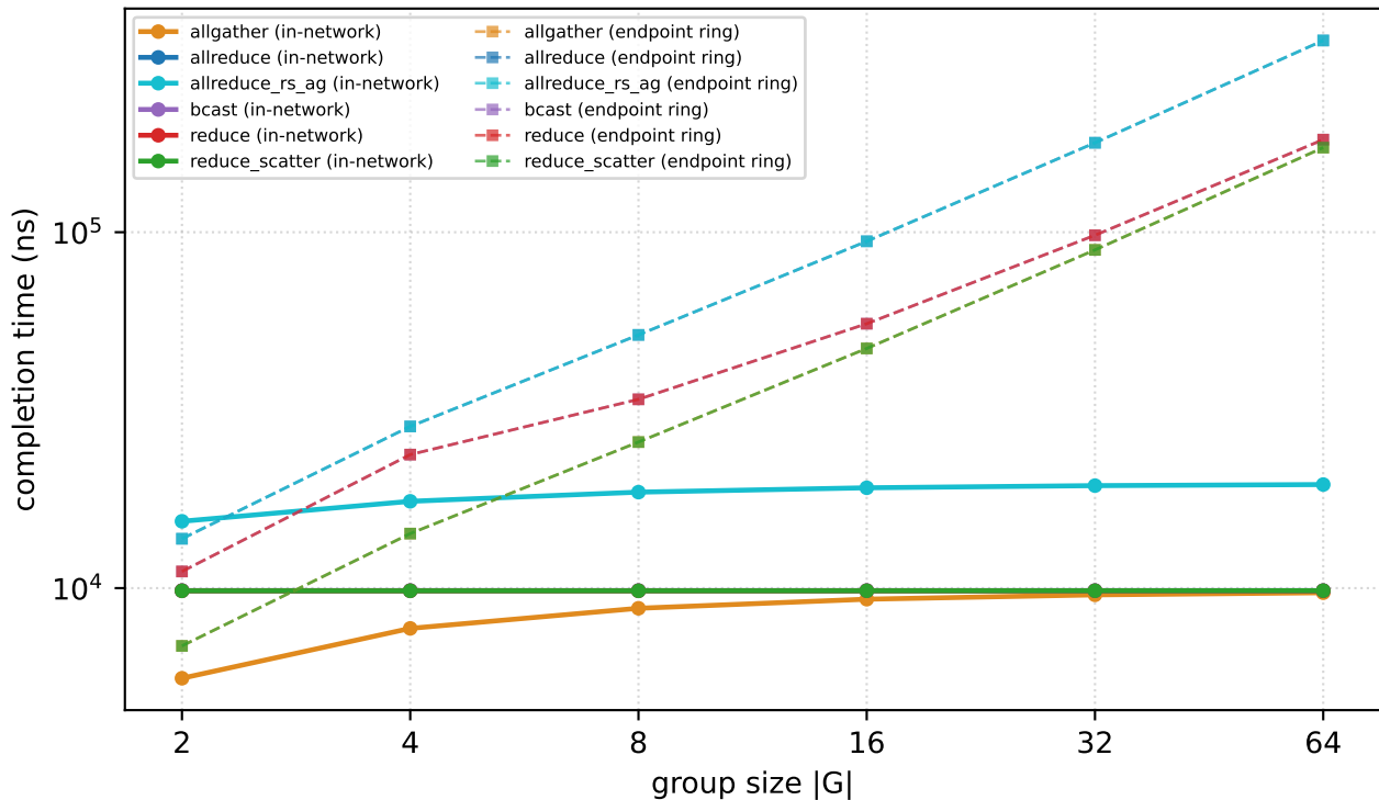
Completion time vs |G| — 4 MiB (pcm-sdk, single-switch, measured) in-network flat = constant-in- |G| (bcast/reduce/allreduce)
