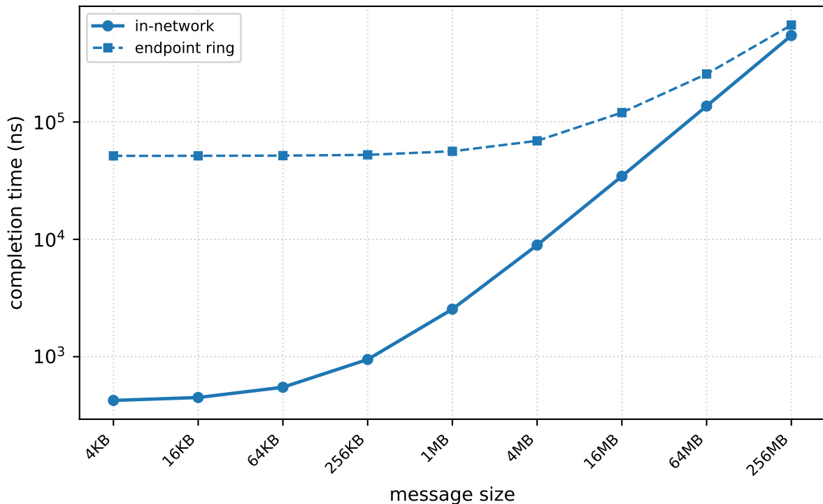
reduce — single_switch, |G|=64 (pcm-sdk, measured)
