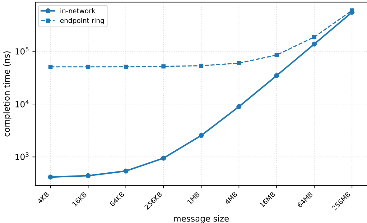
reduce_scatter — single_switch, |G|=64 (pcm-sdk, measured)
