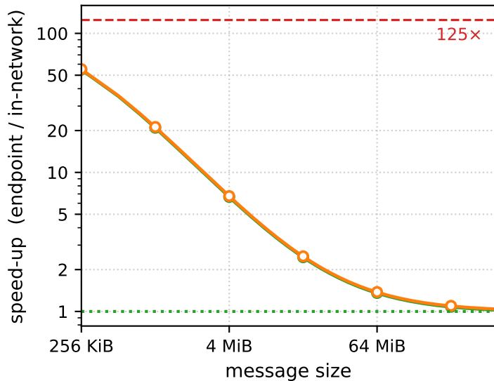
(a) single switch, d = 1
