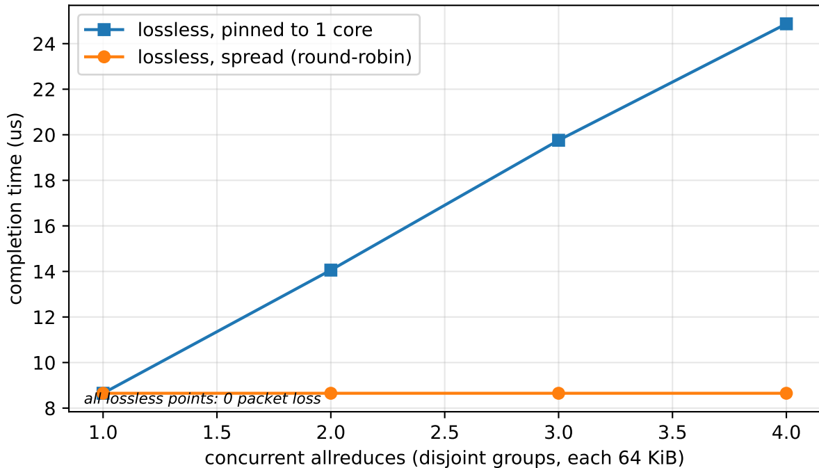
Single-core backpressure: lossless carries the hotspot (0 drops)
