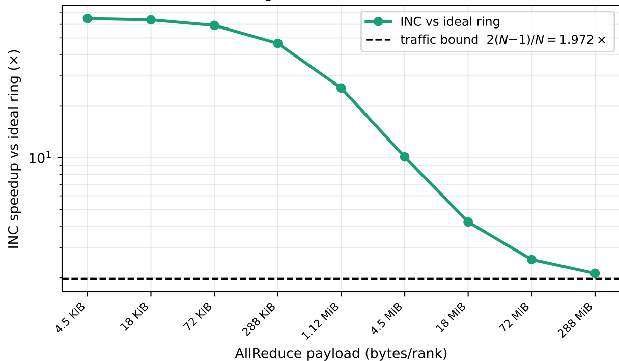
Convergence to the traffic bound
