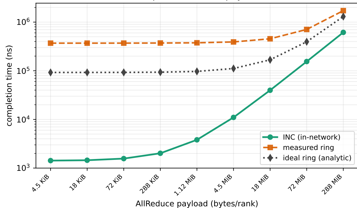
Completion time vs payload
