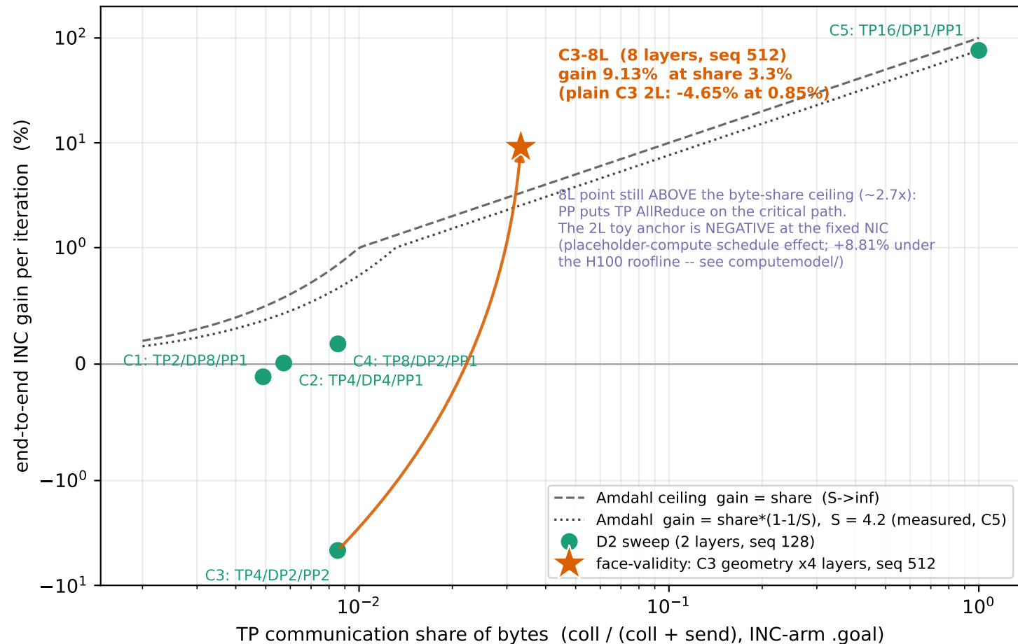
Face-validity: end-to-end INC gain vs TP share at larger block geometry C3 parallelism (TP4/DP2/PP2, 16 ranks) -- 2-layer/seq-128 toy vs 8-layer/seq-512 re-measured 2026-07-14, pcm-sdk (run-only), -intranode_linkspeed 3600000
