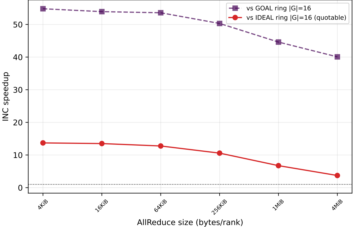
INC speedup vs message size (GOAL-ring level inflated by per-step ACK-leg completion semantic; red = vs analytic ideal ring — see README)
