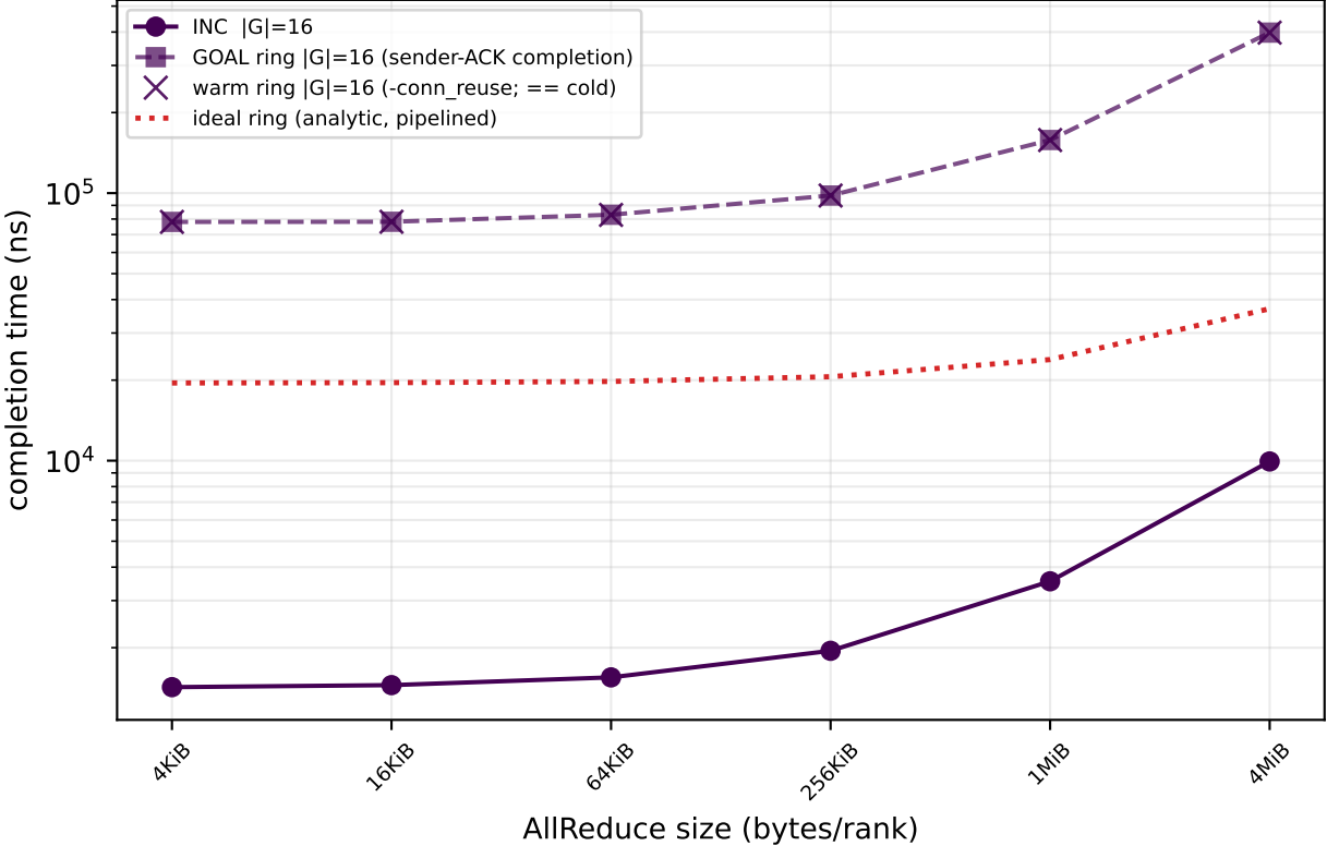
Completion: INC vs ring (measured + analytic ideal)
