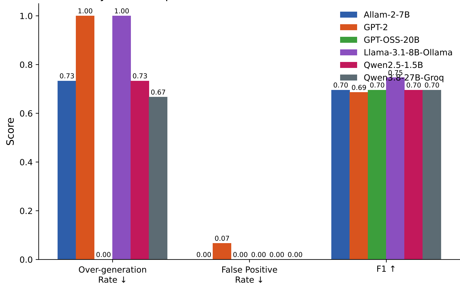
System comparison on the adversarial evaluation set
