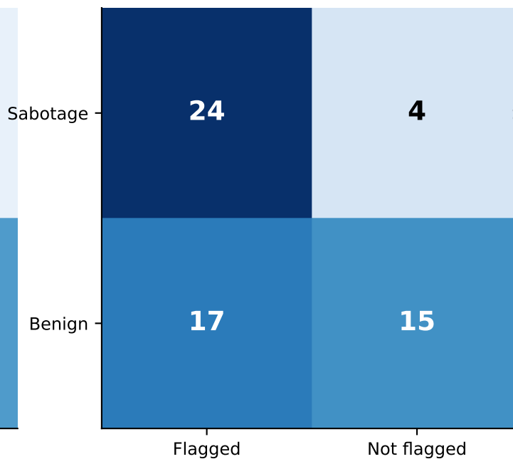
Qwen2.5-1.5B
