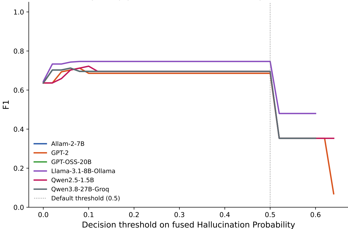
Hybrid pipeline F1 vs. threshold, all systems
