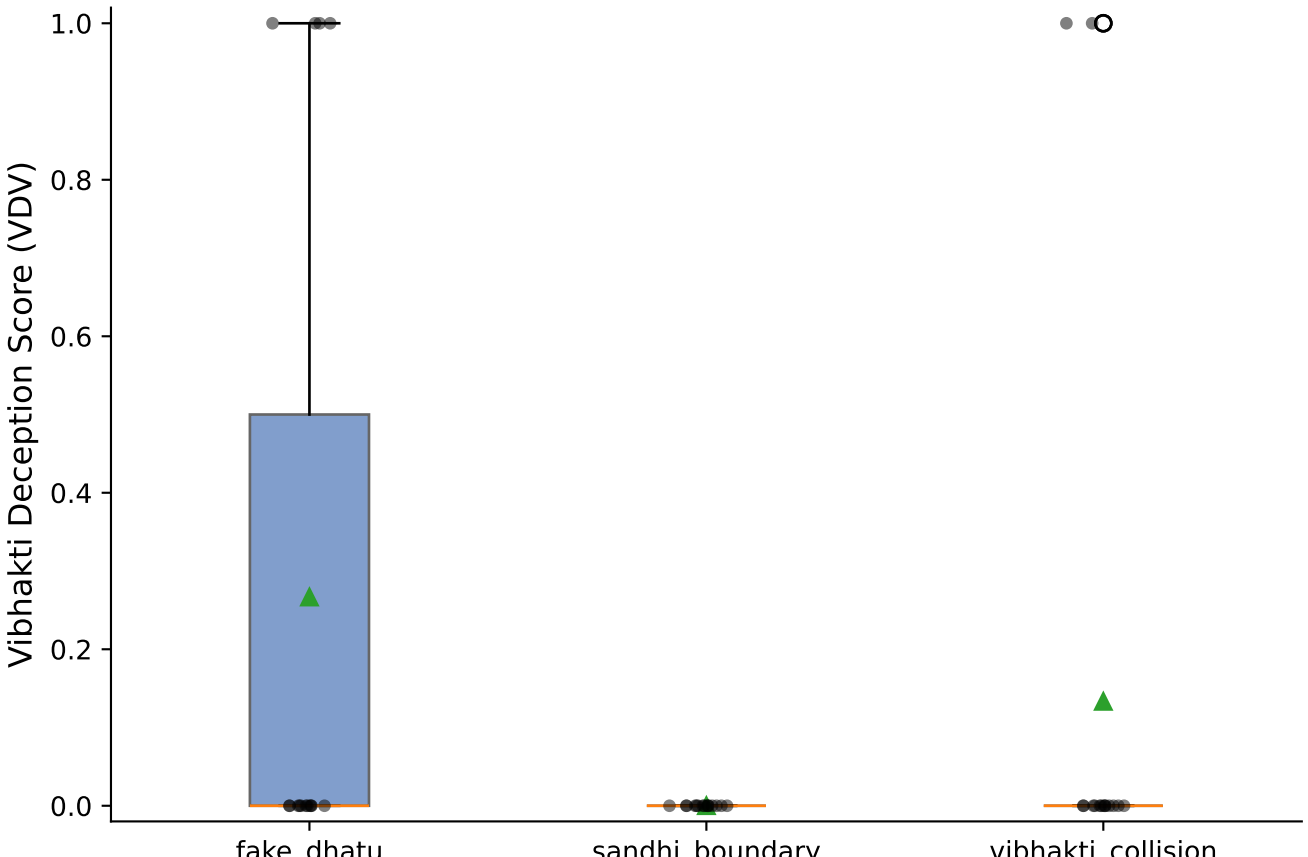
Vibhakti Deception Score (VDV) by adversarial trap type
