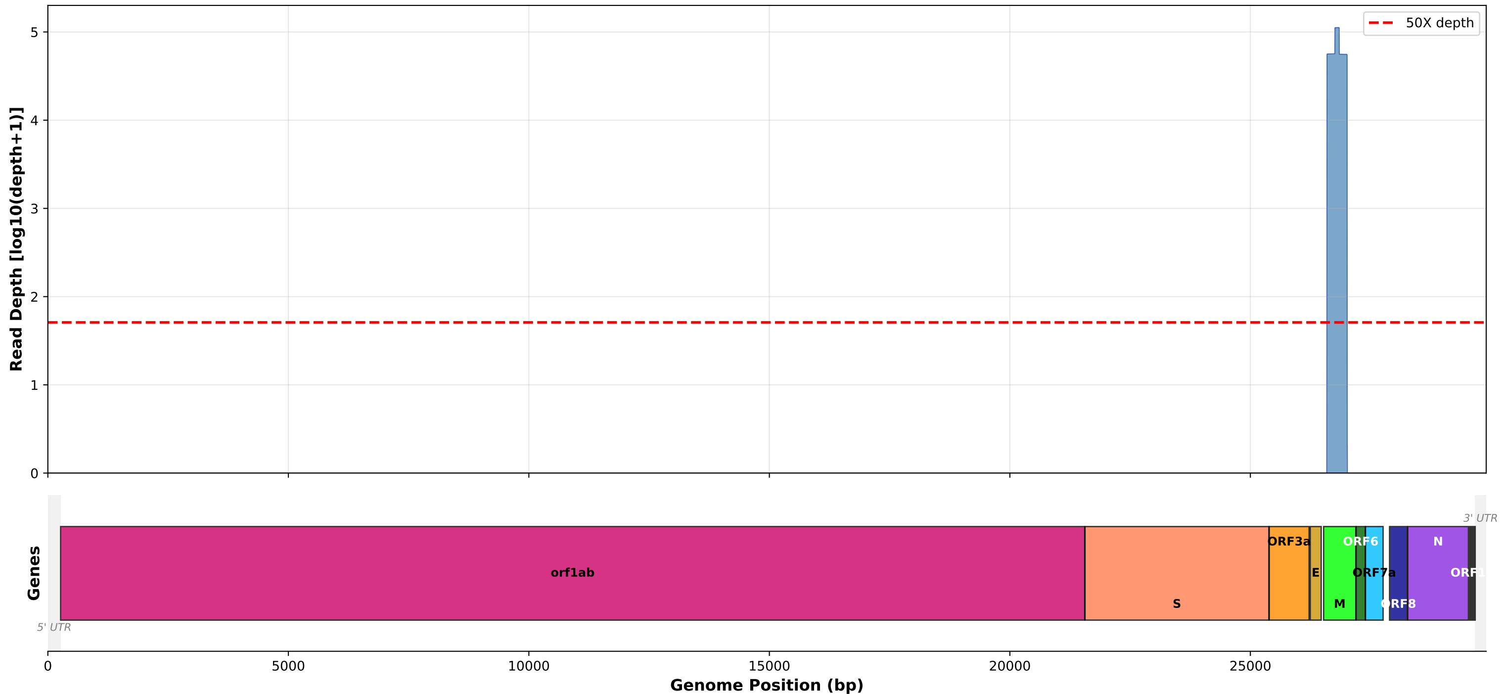
Coverage Map with Gene Annotations
